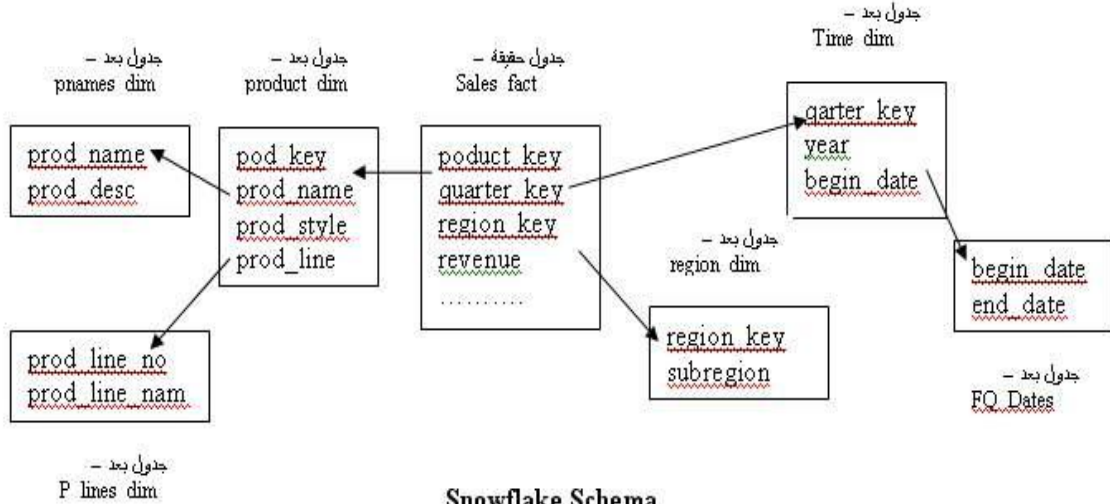
Snowflake Schema
